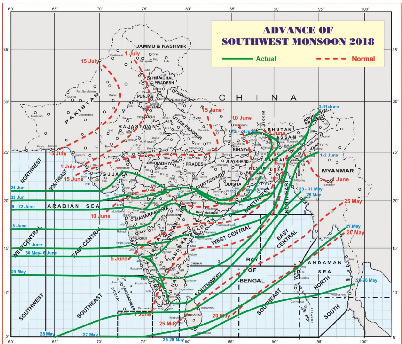
Fig: Advancement of South West Monsoon-2018 and Northern Limit of Monsoon (NLM) as on 24 th June 2018
