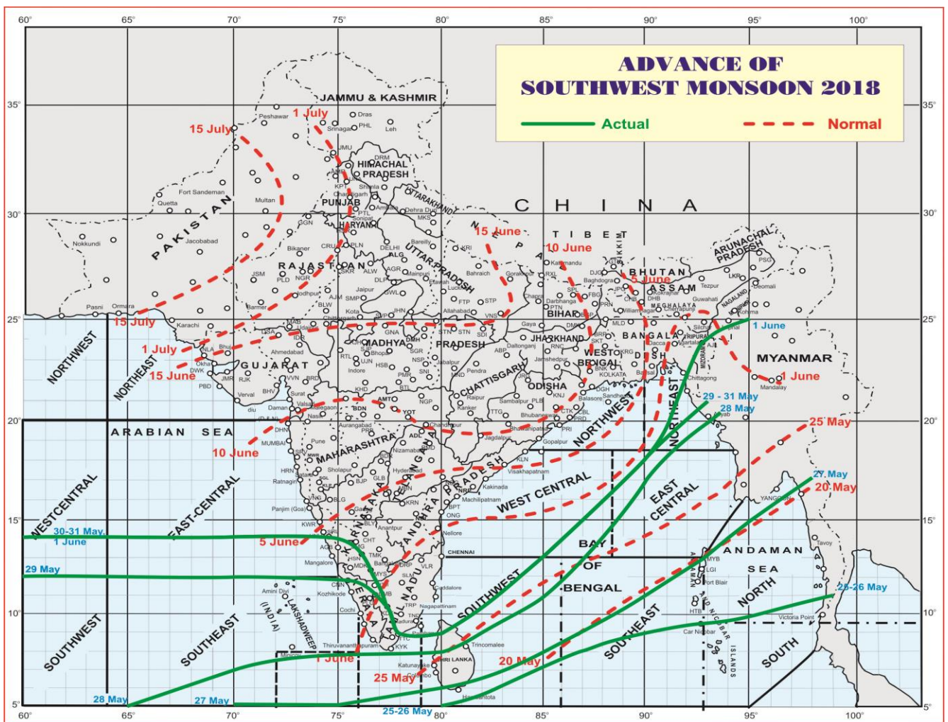
Fig: Advancement of South West Monsoon-2018 and Northern Limit of Monsoon (NLM) as on 01 June 2018
