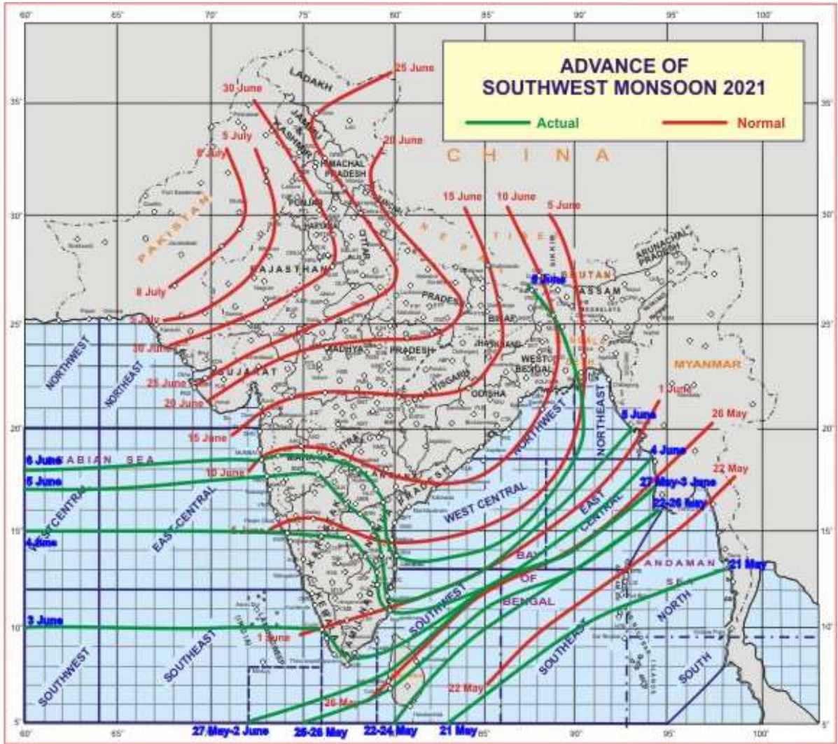
Fig 1: Advancement of Southwest Monsoon 2021
