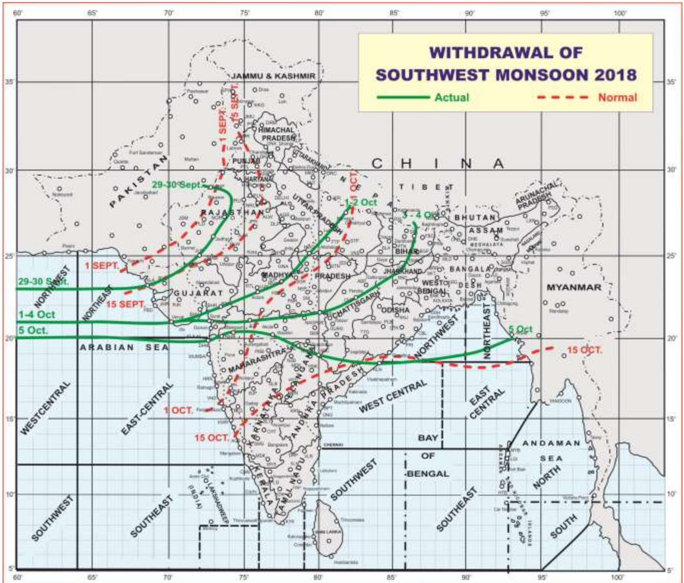
Fig: Withdrawal of South West Monsoon-2018 and Withdrawal Line as on 05 October 2018
